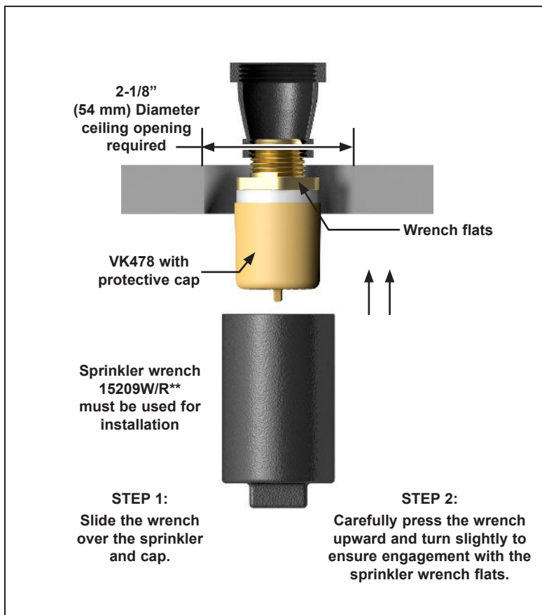
Figure 1: Sprinkler Installation and Correct Use of Wrench
