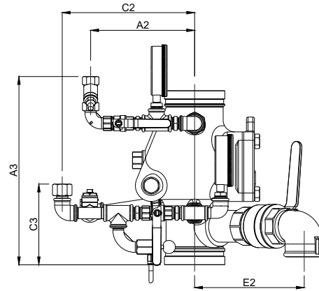
Fig 5.1.2 - Side view
