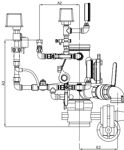
Fig 5.5.2 - Side view
