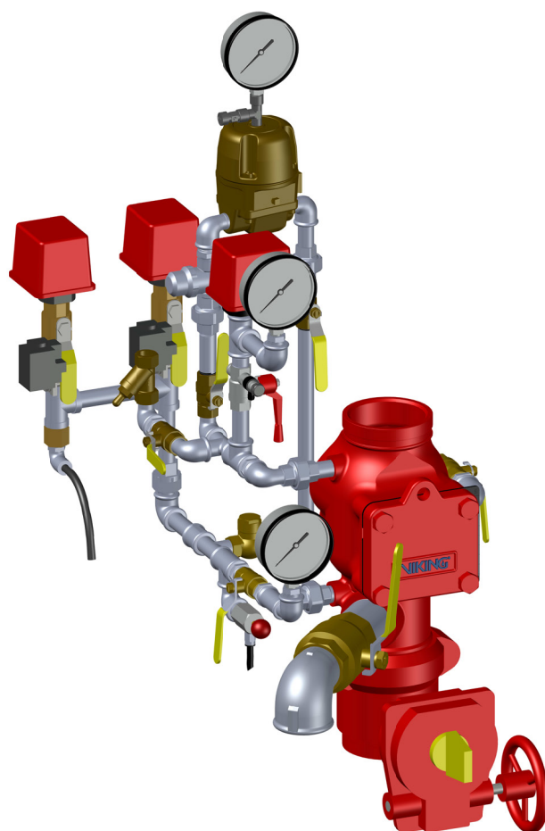
Fig. 3.2.3.b - DRV-1 with accelerator (Norwegian market)
