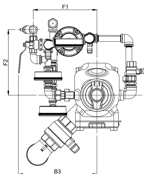
Fig 5.2.2 - Plan view
