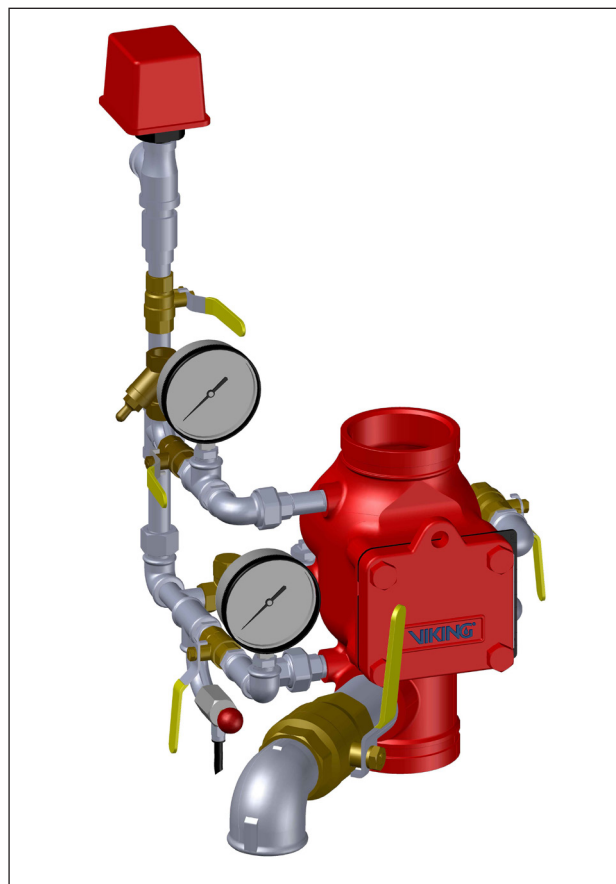
Fig 1.1 - DRV-1 with pressure switch (Image for illustration purposes only)
