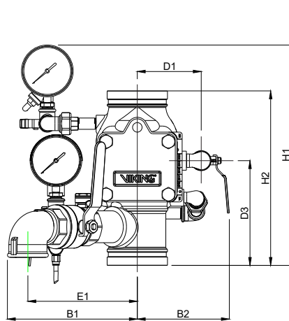
Fig 5.1.1 - Front view
