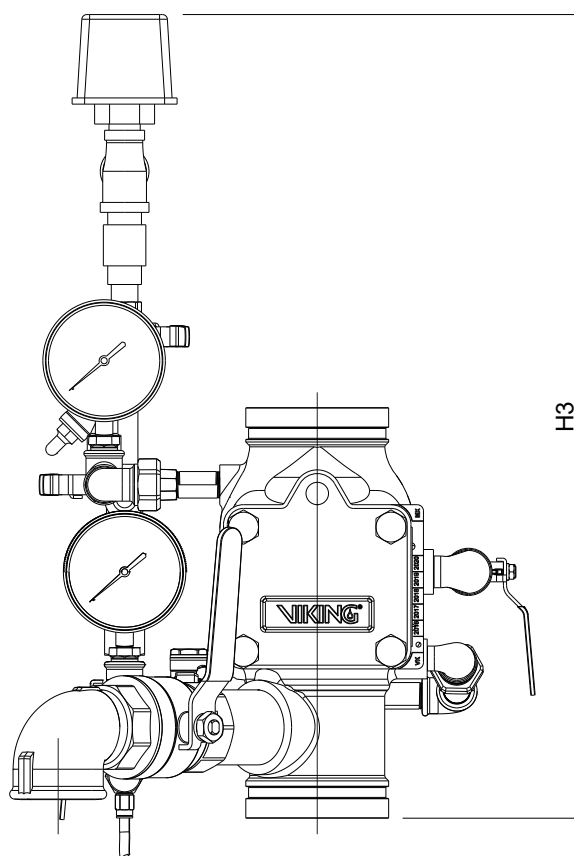
Fig 5.4.1 - Front view (standard trim shown)
