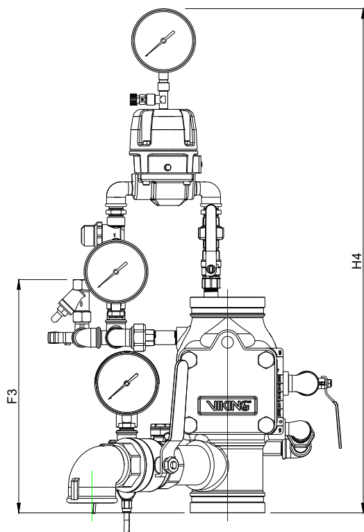
Fig 5.2.1 - Front view
