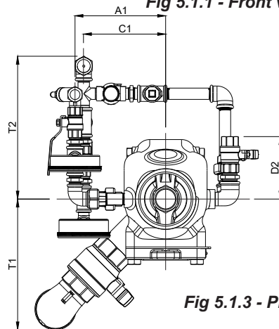
Fig 5.1.1 - Front view
